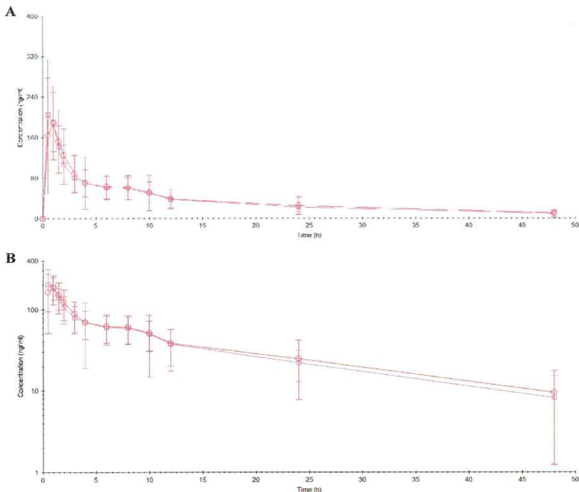
Figure 2: (A) Mean plasma concentration-time curves for TFV (n=39) following single-dose administration of test and reference (1 x 300 mg) tablets. Test= square and reference=circles. (B) Mean plasma log-concentration time curves for TFV (n=39) following single-dose administration of test and reference (1 x 300 mg) tablets. Test= square and reference=circles.
