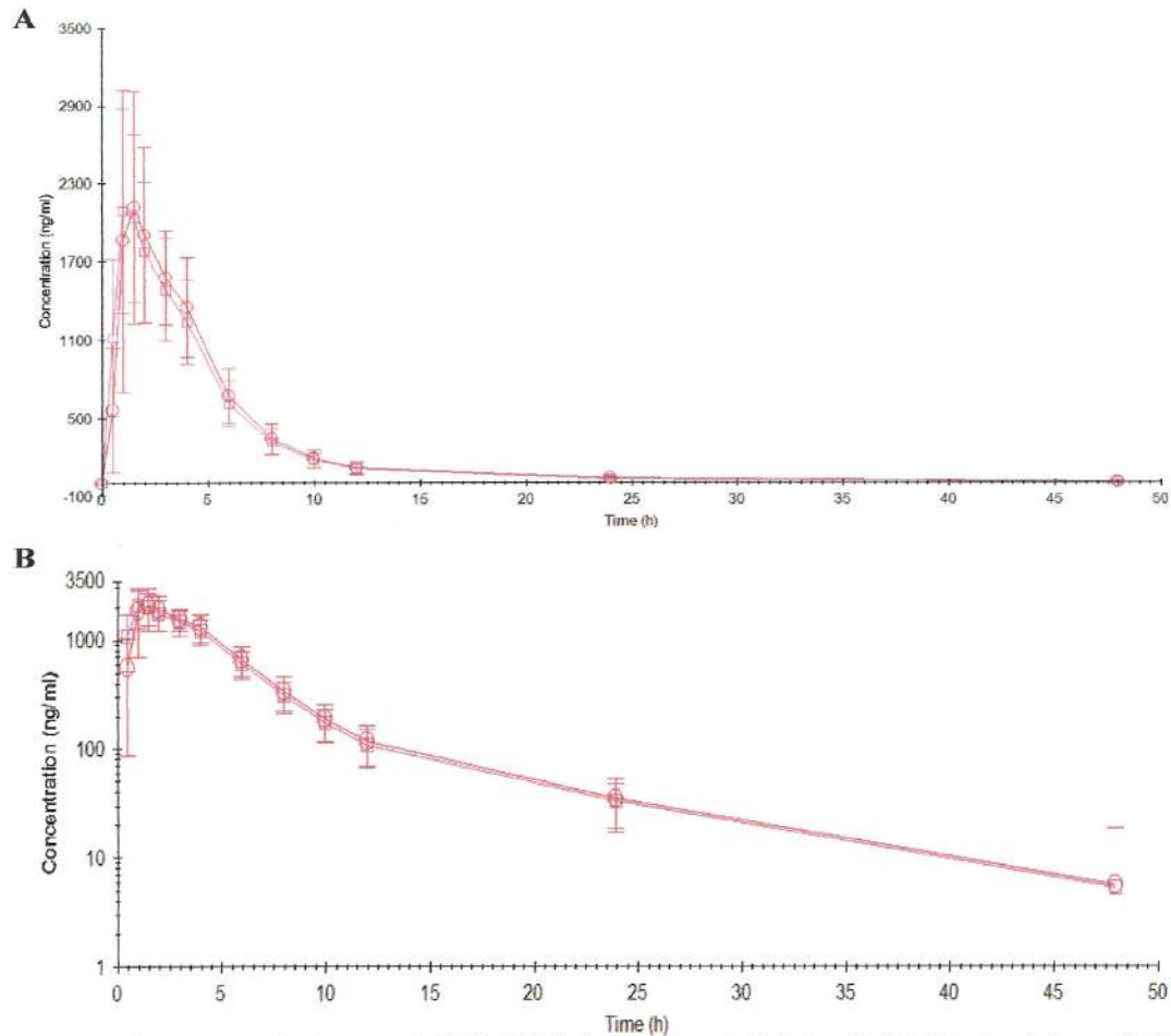
Figure 3: (A) Mean plasma concentration-time curves for 3TC (n=39) following single-dose administration of test (1 x 300 mg) and reference (2x 150 mg) tablets. Test= square and reference= circles. (B) Mean plasma log-concentration time curves for 3TC (n=39) following single-dose administration of test (1 x 300 mg) and reference (2x 150 mg) tablets. Test= square and reference= circles.
